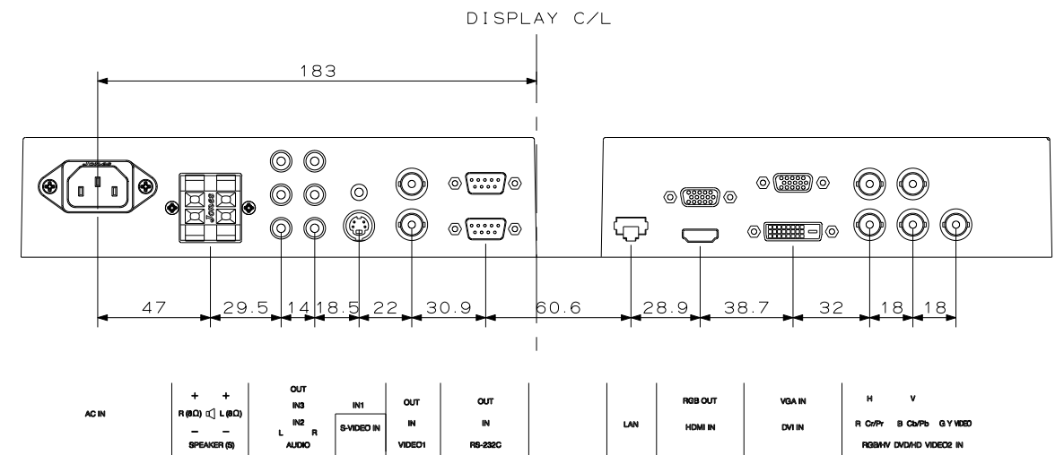
I/O TERMINAL
