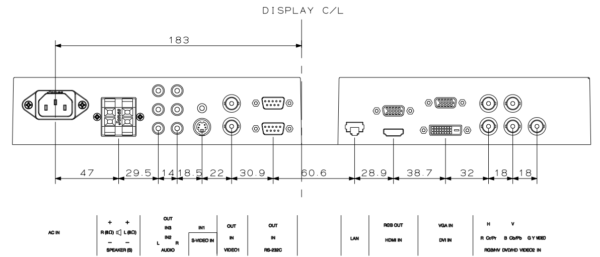
I/O TERMINAL
