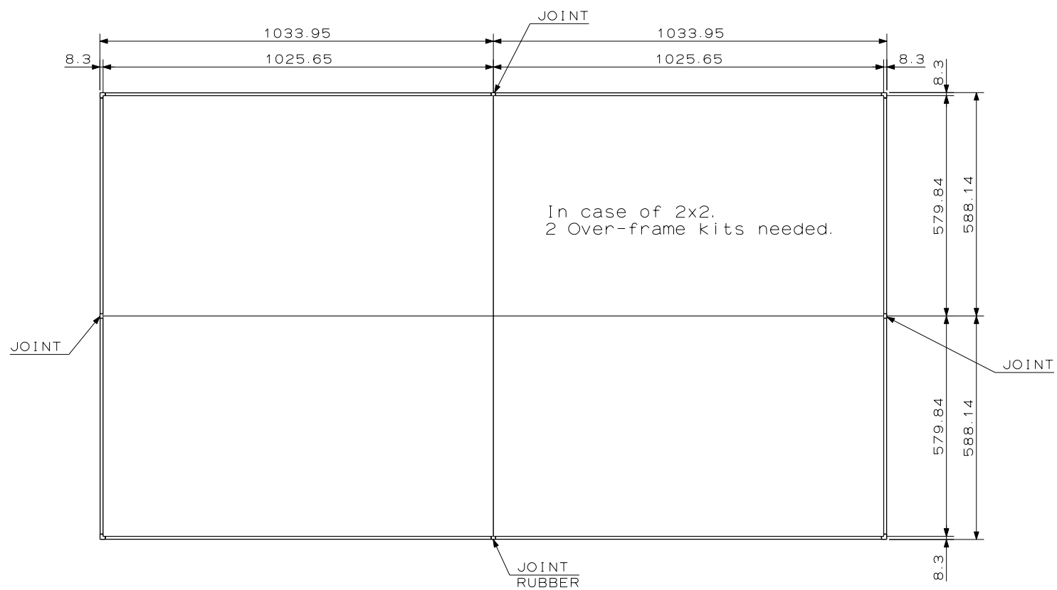
X461UN with Over-frame kit OUTLINE DRAWING
