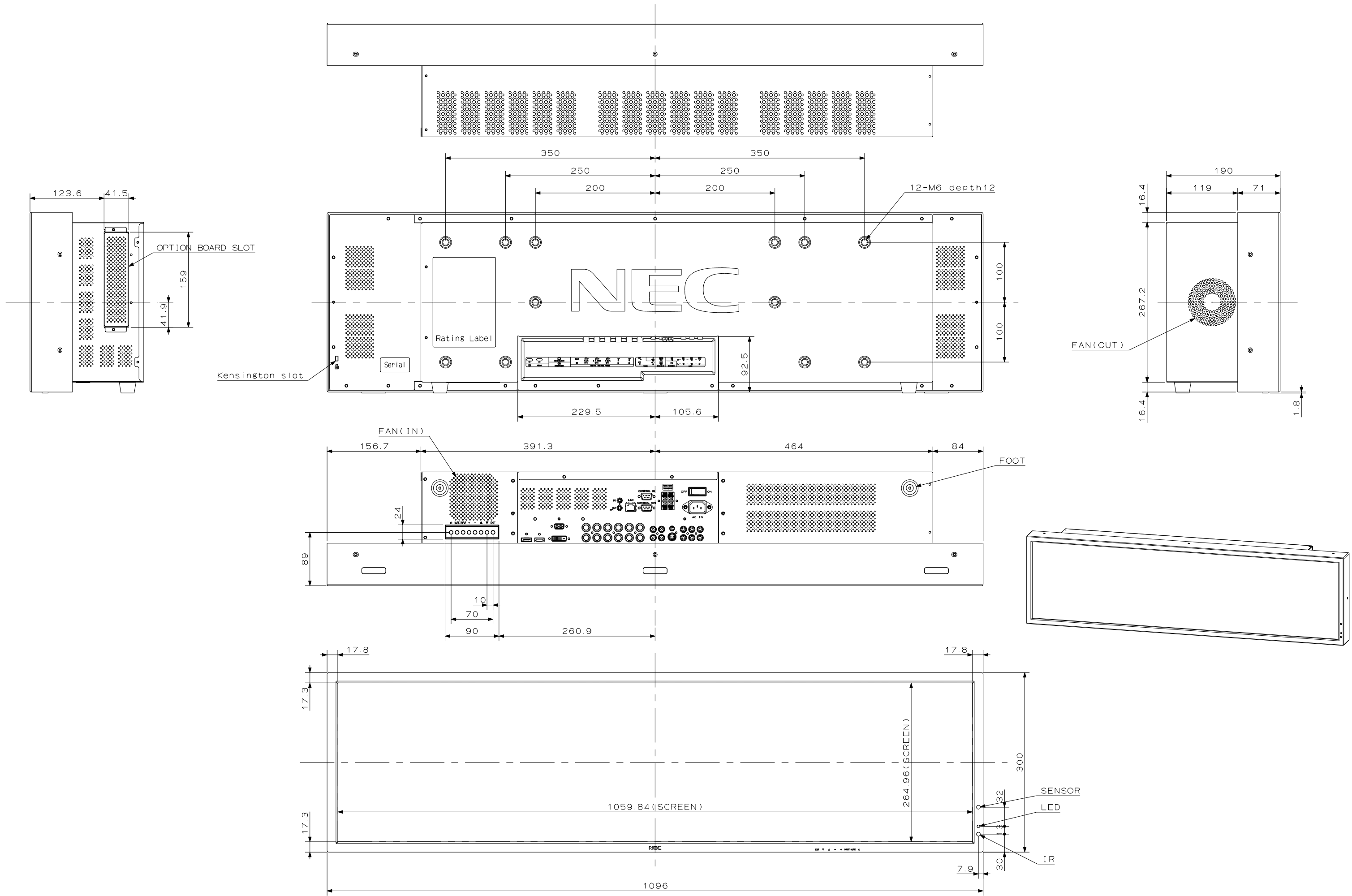
X431BT OUTLINE DRAWING v1.0 2010.01.12 NEC DISPLAY SOLUTIONS, LTD.
