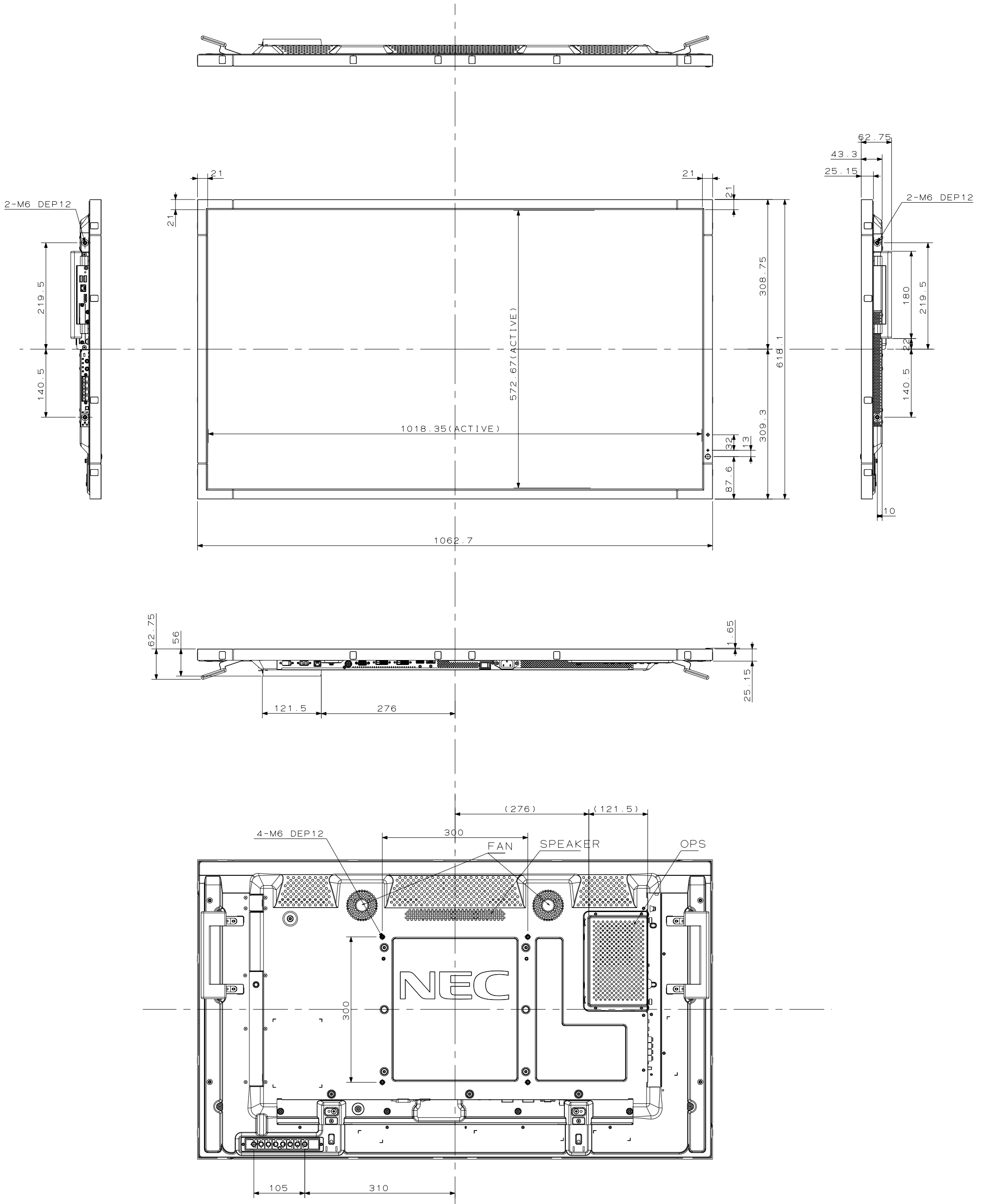
X461S with OPS OUTLINE DRAWING 2011/04/25
