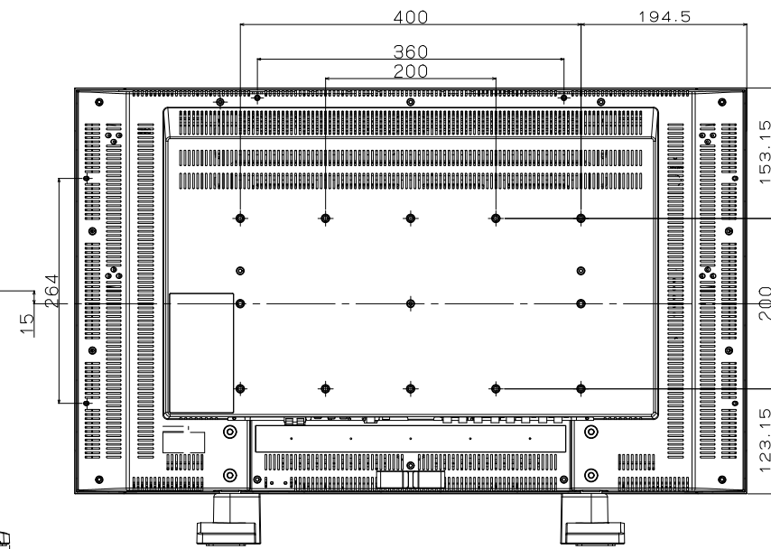
LCD3215 with ST-3215 Outside Drawing
