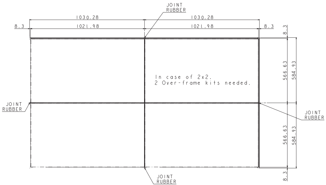
X464UNS with KT-46UN-OF4 OUTLINE DRAWING NEC Display Solutions, Ltd
