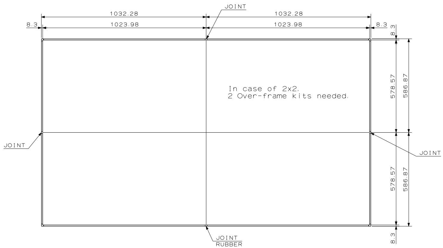
X463UN with KT-46UN-OF2 OUTLINE DRAWING
