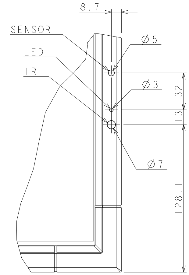
DETAIL A SCALE 1/2
