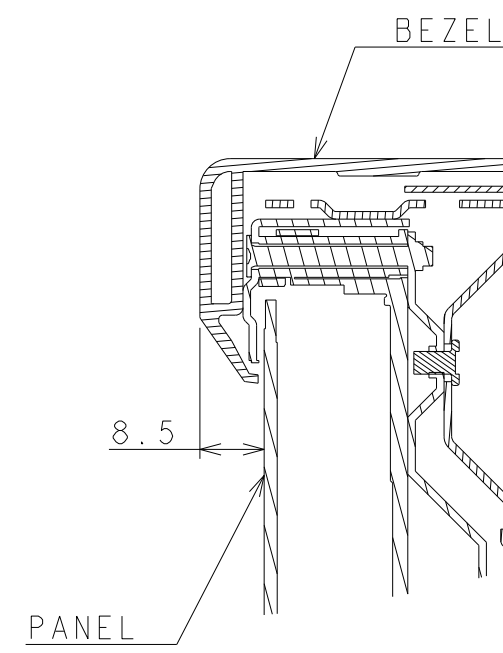
section B-B scale 1/1
