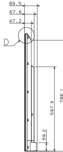
Section A-A Scale 1/1
