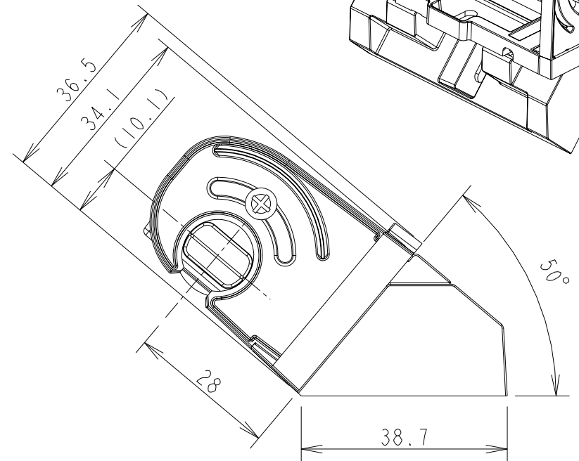
KT-RC2 Sensor Unit with spacer outline drawing 2016.05.13 NEC Display Solutions, Ltd.
