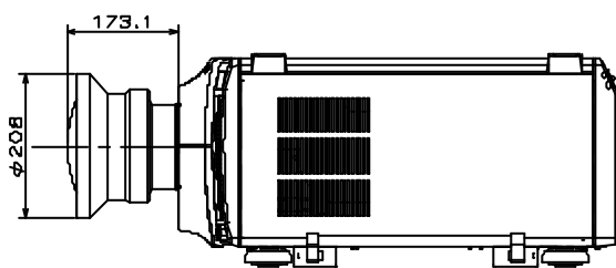
SX6000DJ/SX4000DJ/XT5100J/XT4100J 取付時
