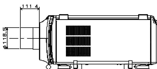
SX6000DJ/SX4000DJ/XT5100J/XT4100J 取付時
